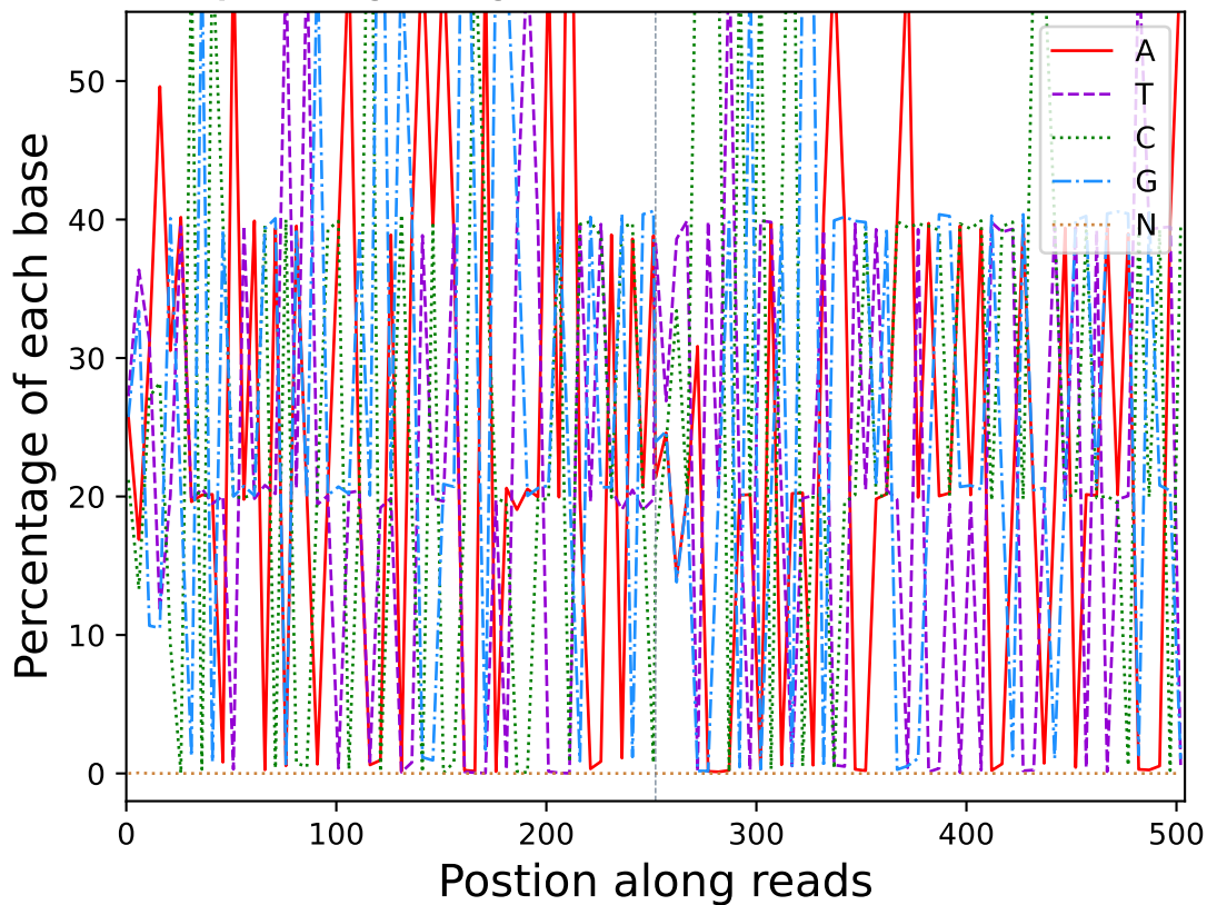
Base percentage along reads (R10101)
